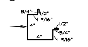
15 OUTSIDE CORNER
