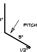
10 SIDEWALL
