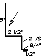
11 SNOW BREAK
