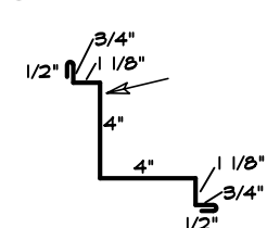
15 OUTSIDE CORNER
