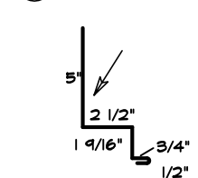
11 SNOW BREAK
