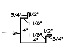
15 OUTSIDE CORNER
