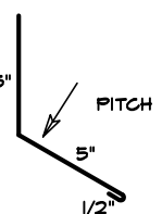
10 SIDEWALL
