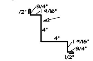
15 OUTSIDE CORNER
