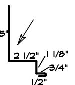
11 SNOW BREAK
