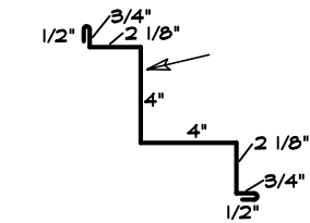
15 OUTSIDE CORNER
