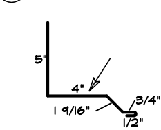
11 SNOW BREAK
