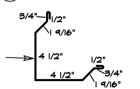
16 BASE TRIM
