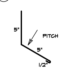
10 SIDEWALL
