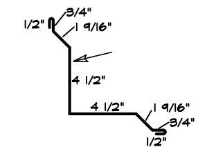
15 OUTSIDE CORNER
