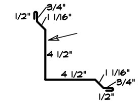
15 OUTSIDE CORNER
