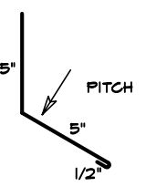
10 SIDEWALL
