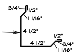
16 BASE TRIM
