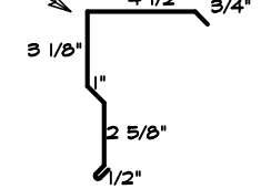
4a 2X6 GABLE
