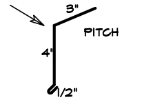
5b 2X4 EAVE
